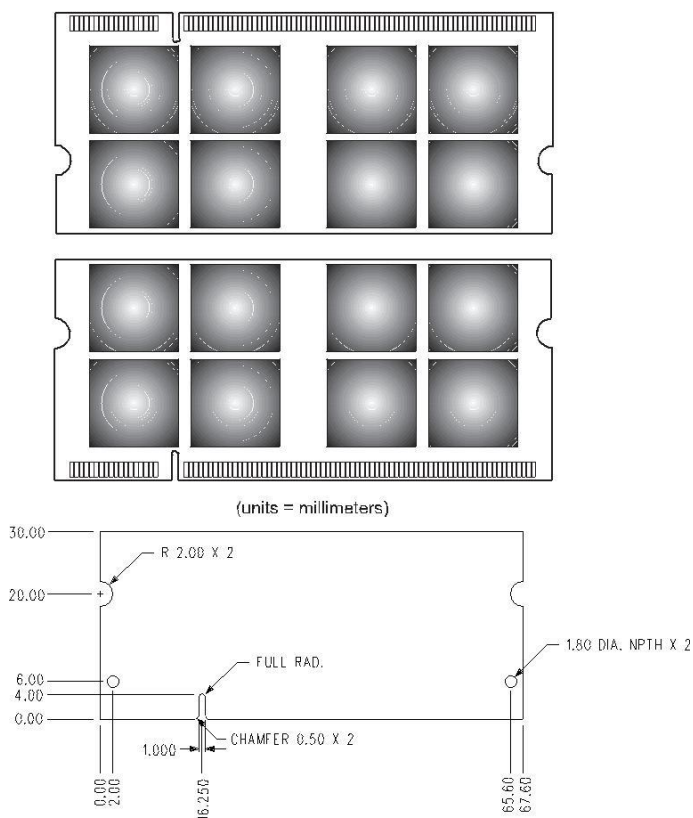
Figure 1: DDR2 2G 800 1.8V SO-DIMM
